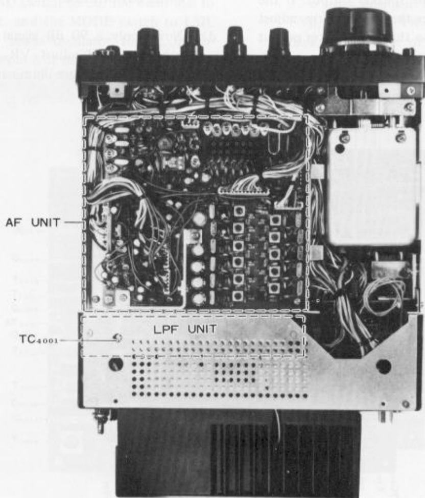
BOTTOM VIEW
